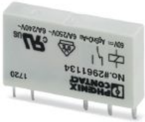
Plug-in miniature power relay, with multi-layer gold contact, 1 PDT, input voltage 60 V DC
