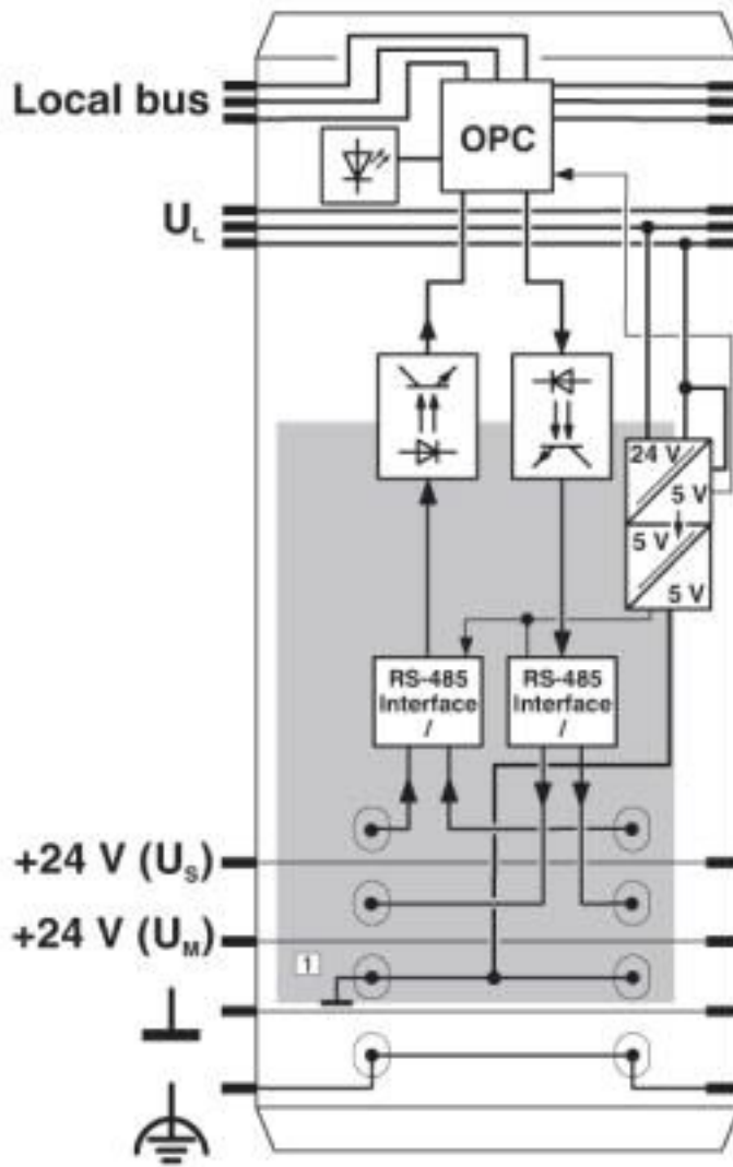
Internal wiring of the terminal points
