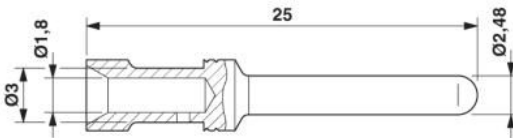
Dimensional drawing
