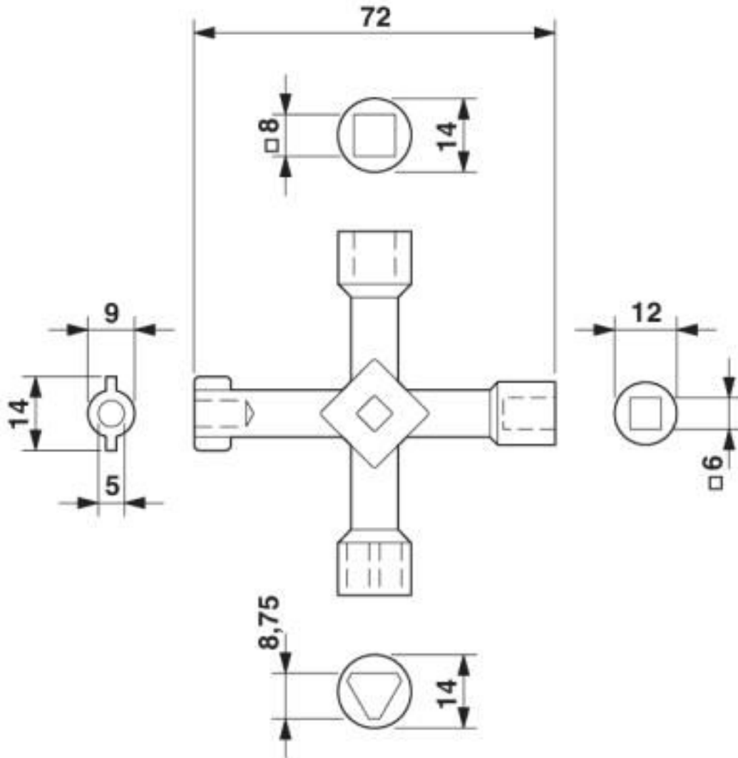
Dimensional drawing
