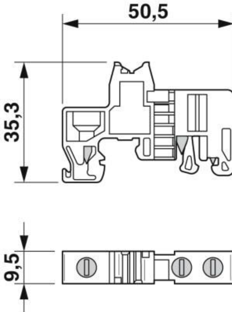
Dimensional drawing
